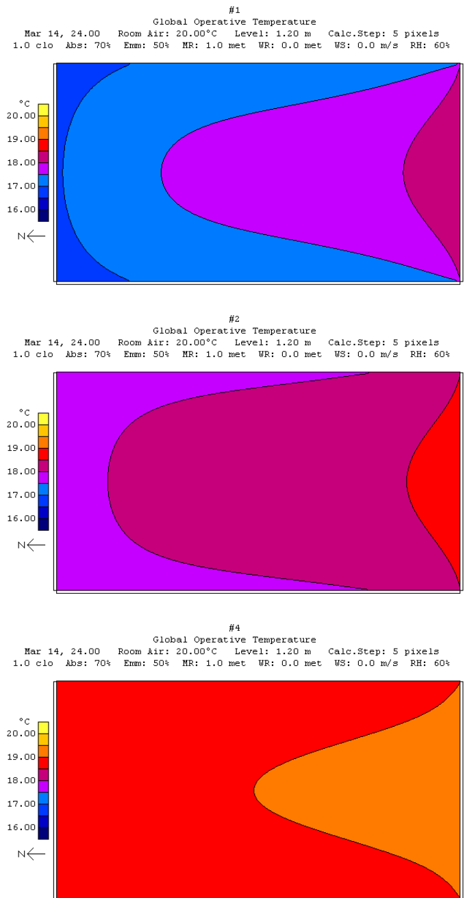
Figure 5.35 Global operative temperature at an outside temperature of -5^{\circ}\text{C} , no solar radiation, for three glazing U -values: 1.65 (top), 1.14 (middle) and 0.67 \text{ W/m}^2\text{K} (bottom).
