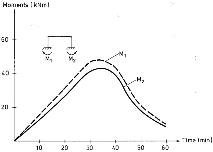
Figure 6.29 Moments at the fixed supports
