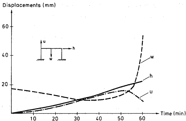
Figure 6.27 Calculated displacements
