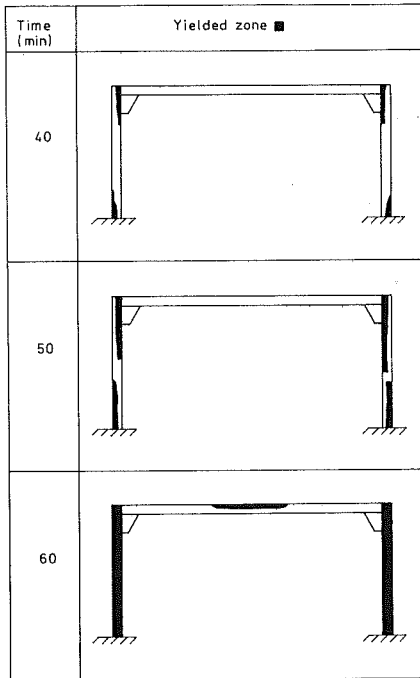
Figure 6.28 Spread of yielded zones
