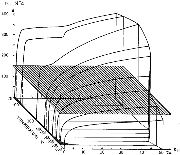
Figure 3.9 Stress-strain-temperature surface
