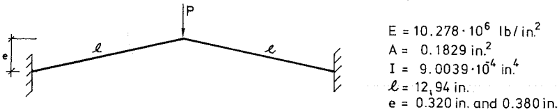
Figure D.6 Williams's toggle
