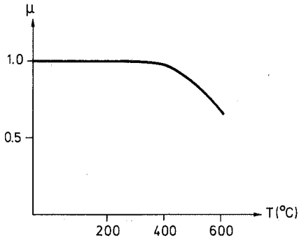
Figure C.2 Variation of the parameter \mu in Eq. (C.1) with temperature
