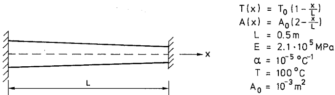
Figure D.12 Fixed bar
