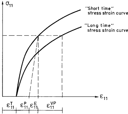
Figure 3.1 Strain components
