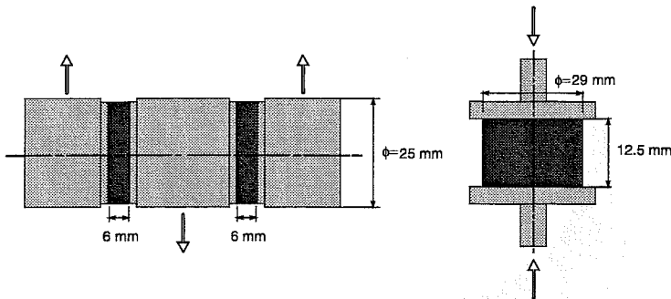
Figure 5.13: Double shear and compression specimens.
