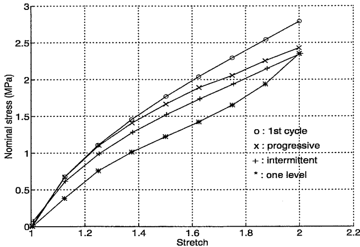
Figure 5.3: Stationary average loading values for the three different conditioning procedures and first cycle data.
