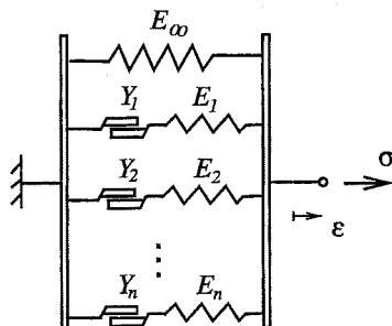
Figure 10.1: The generalized frictional solid model.
