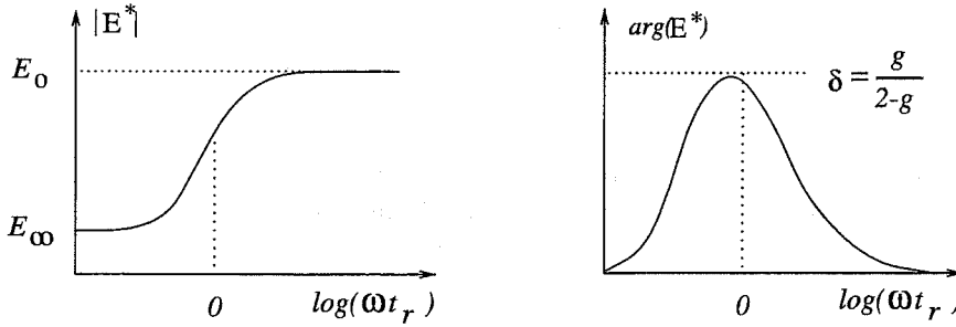
Figure 9.17: Zener model; frequency dependence of the complex modulus for g \leq 0.5 .
