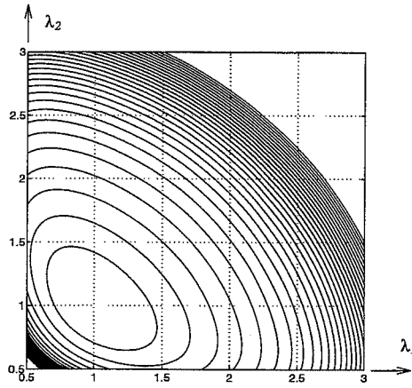
Figure 5.9: Strain energy function for the three-parameter model.
