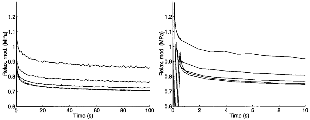
Figure 8.8: Relaxation modulus in shear i.e. relaxation stress divided by the magnitude of the strain steps; \kappa_s=[0.2 \ 0.4 \ 0.6 \ 0.8 \ 1.0] for 100 s and a closer view of the first 10 s. The largest relaxation modulus corresponds to the smallest strain step.
