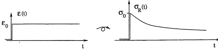
Figure 9.2: Relaxation behavior; decreasing stress as response to a strain step.
