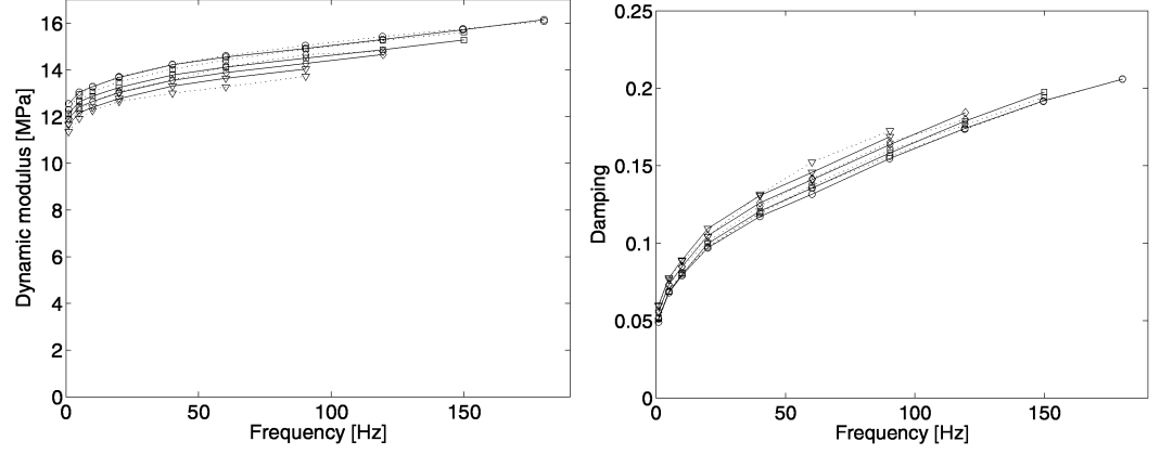
Figure 18: Dynamic shear modulus (left) and damping (right) of SamiIII. Solid line: material model. Dotted line: experimental data. \circ : \kappa_0 = 0.667\% ; \nabla : \kappa_0 = 2\% ; \square : \kappa_0 = 4\% ; \triangle : \kappa_0 = 6.7\% .
