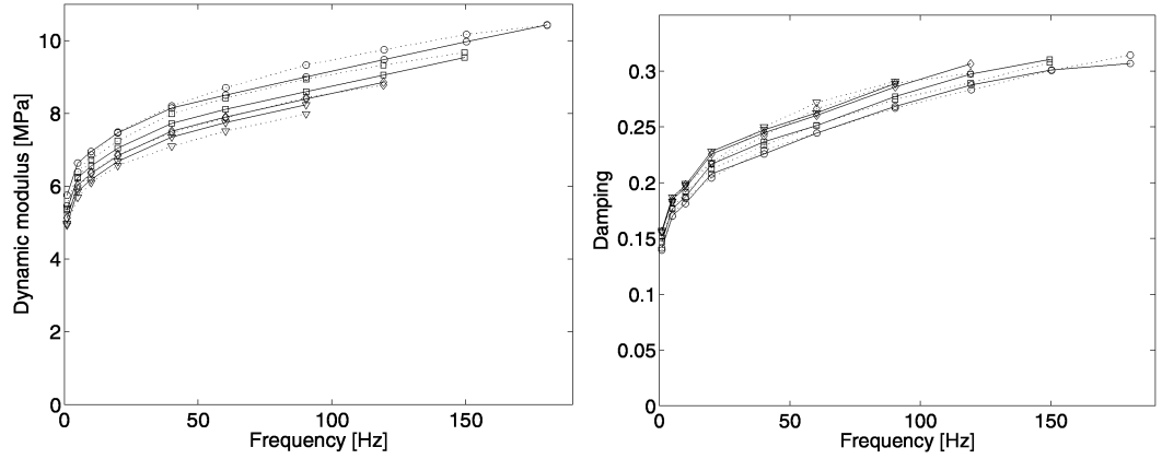
Figure 11: Dynamic shear modulus (left) and damping (right) of HGSD85. Solid line: material model. Dotted line: experimental data. \bigcirc : \kappa_0 = 1\% ; \nabla : \kappa_0 = 3\% ; \square : \kappa_0 = 7\% ; \triangle : \kappa_0 = 12\% .
